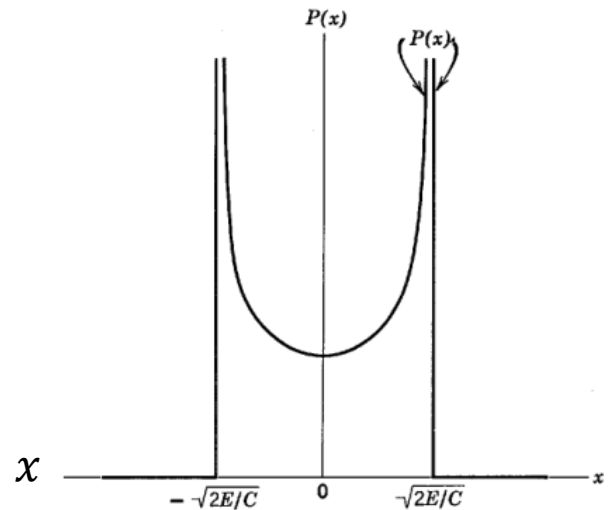
Classical harmonic Oscillator probability P(x)
